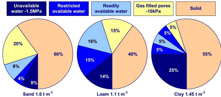
Figure 6 Water availability and volumetric relationships between solid, liquid and gaseous phases for three soils of different texture and density.
